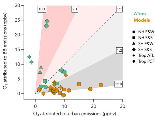
Fig. 5. Concentration-weighted average \text{O}_3 attributed to urban and BB emissions. ATom observations are shown in green (the two markers per symbol are from the two pairs of tracers used to identify air mass influences), and modeling results are shown in brown. The uncertainties are in SI Appendix, Table S3 (observations) and SI Appendix, Table S4 (modeling results).
